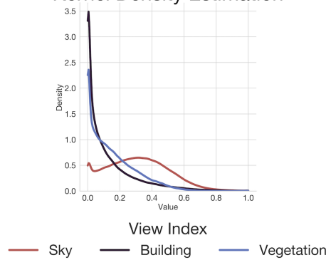
(e) Probability density distribution of view indices across Singapore. The plot shows the relative frequency of different index values [0, 1] for buildings, vegetation, and sky visibility, highlighting the varying urban morphology patterns. Building views show high density at lower values, while sky views demonstrate a bimodal distribution.
