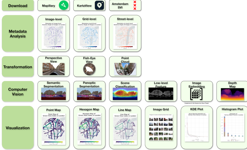
Figure 1: Overview of the framework of ZenSVI package, consisting of five sub-packages: 1) download, 2) metadata analysis, 3) computer vision, 4) image transformation, and 5) visualization.
