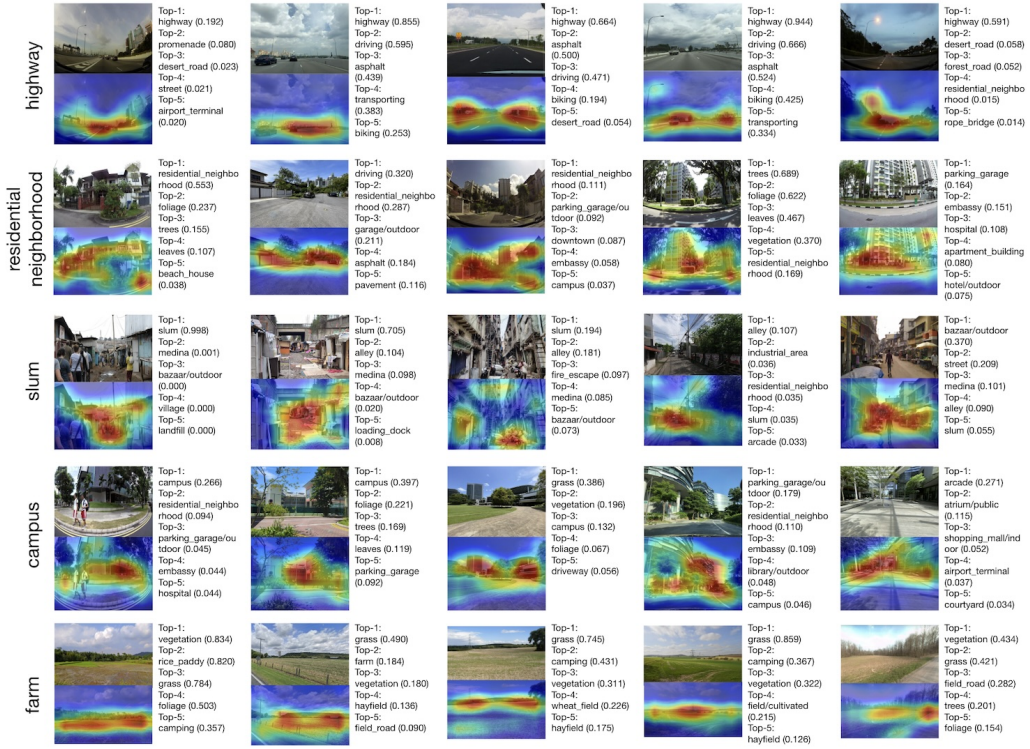
Figure 8: Places365 scene classification examples in five different settings: highway, residential neighborhood, slum, campus, and farm.
