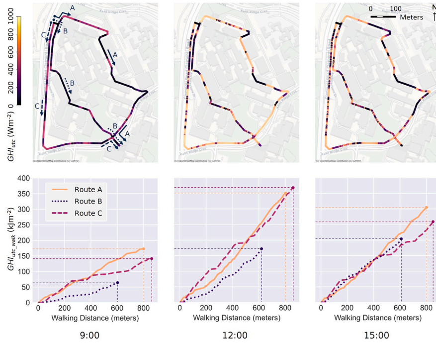
Fig. 19. Maps displaying GHl_{walk} values for each route and line charts illustrating the changes in GHl_{walk} during a walk along each route, comparing results at 9:00, 12:00, 15:00 on January 1, 2024. Basemap: © OpenStreetMap contributors, © CARTO.
