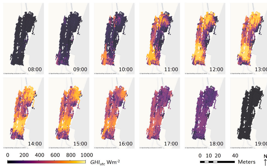
Fig. 17. Time-series high-resolution maps of GHI_{UTC} from 08:00 to 19:00 on January 1, 2024 at one-hour intervals. Basemap: © OpenStreetMap contributors, © CARTO.
